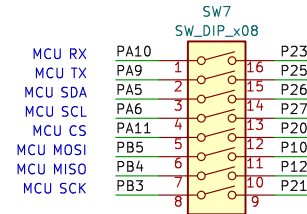
Connector to Bridge MCU and FPGA
