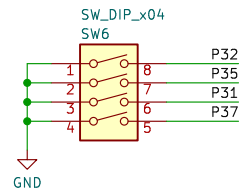
DIP Switches (Use Internal Pull-up Resistors)
