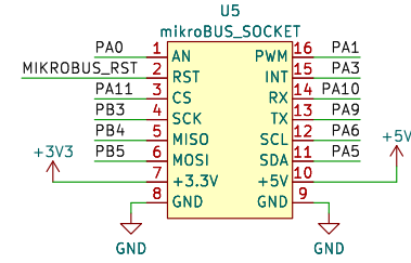
Connector to Bridge MCU and FPGA
