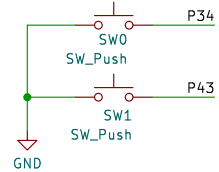
Push Buttons (Use Internal Pull-up Resistors)
